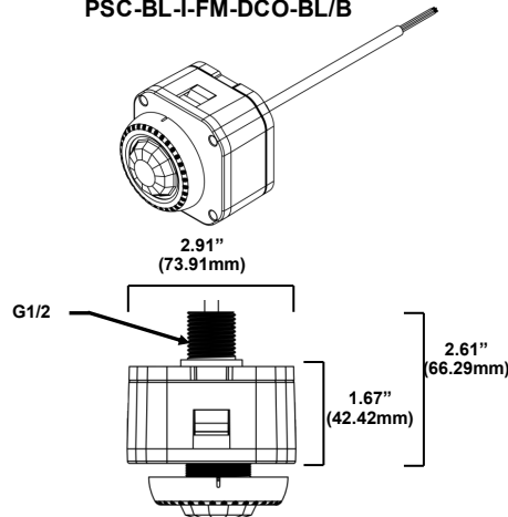
Bottom Mount Housing PSC-BL-I-FM-DC0-BL/B
